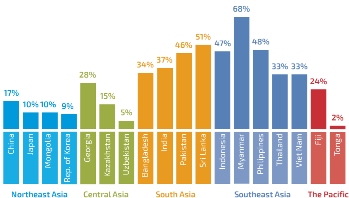
Renewable Share in Total Final Energy Consumption in the selected Asia Pacific Countries, 2016. Source: https://www.ren21.net/wp-content/uploads/2019/05/REN21_Asia_Report_2019_Web.pdf
